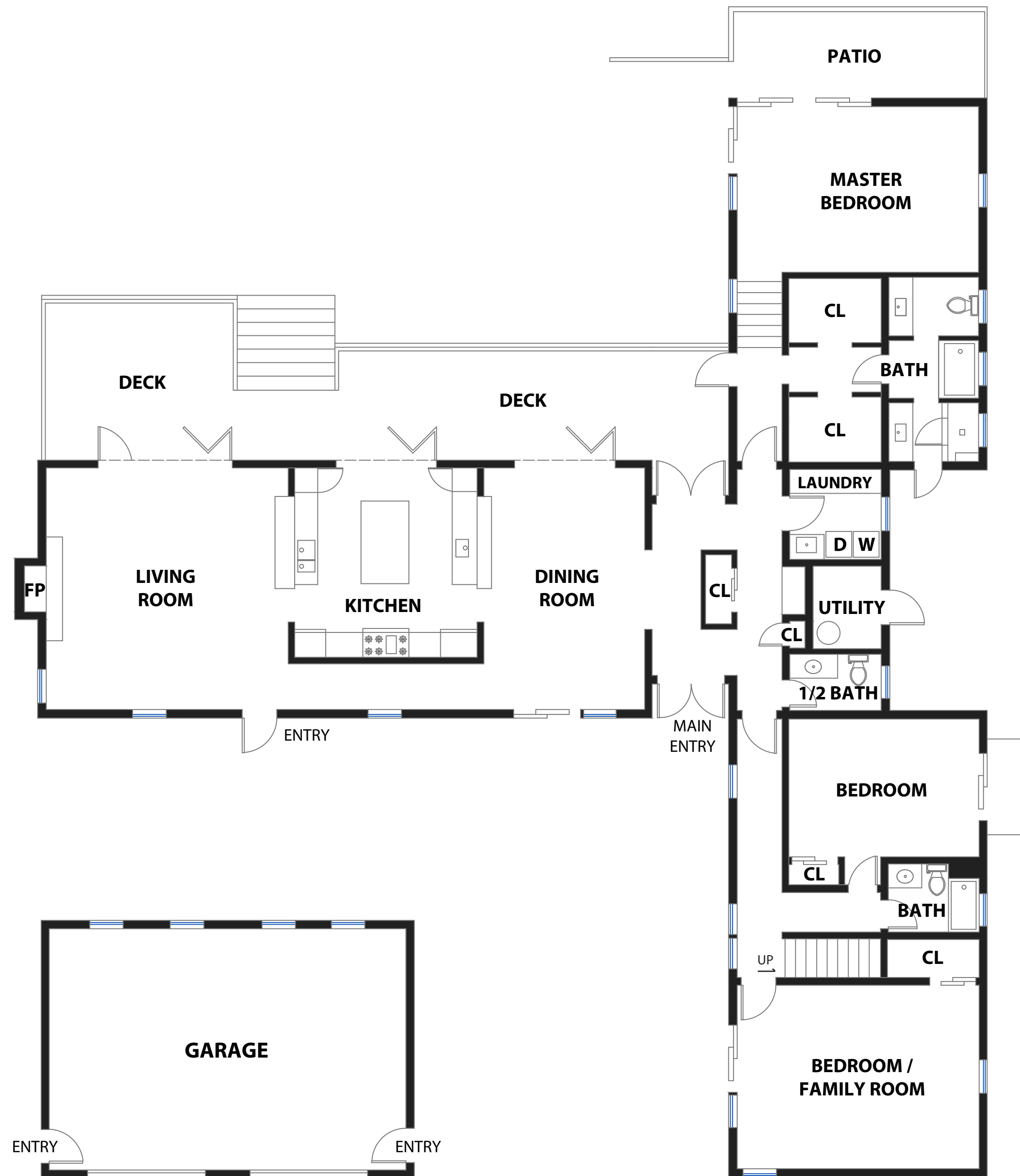
MAIN LEVEL
